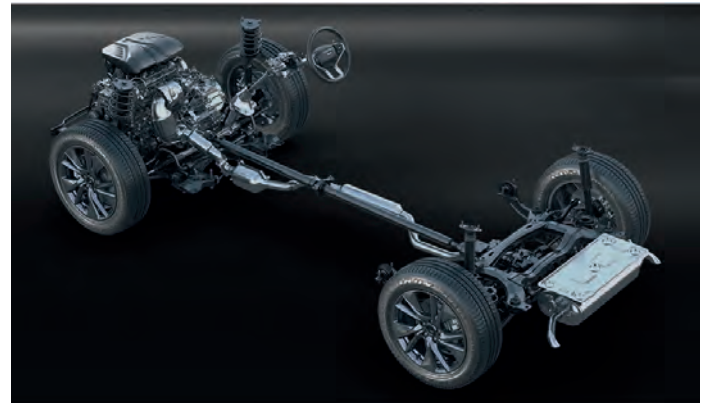
Front Macpherson Rear Multi-link Independent Suspension + AWD
